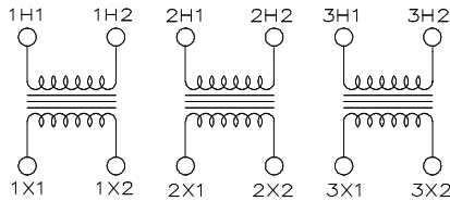
Connection Diagram
