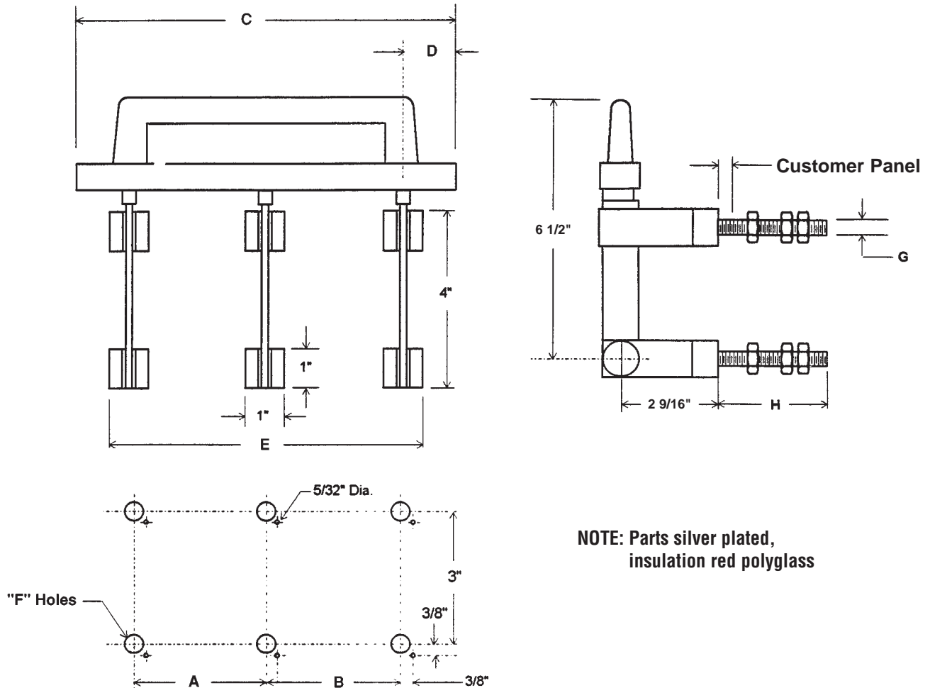
Panel Drilling
