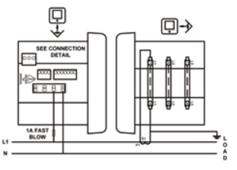
1-phase 2-wire
