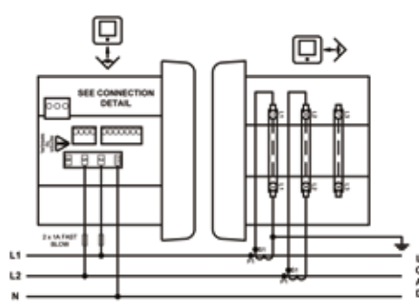
1-phase 3-wire
