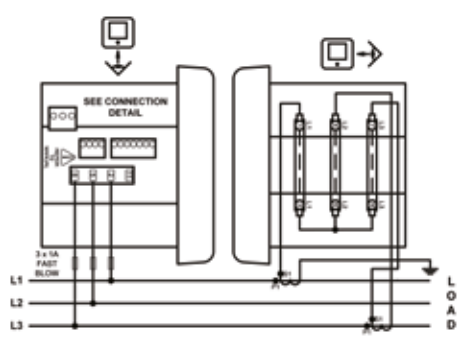
3-phase 3-wire unbalanced
